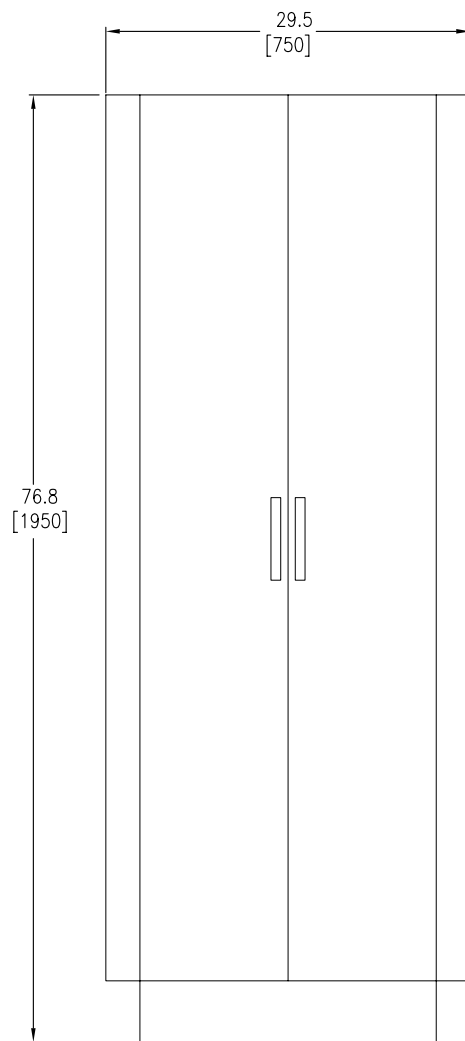
FRONT VIEW
