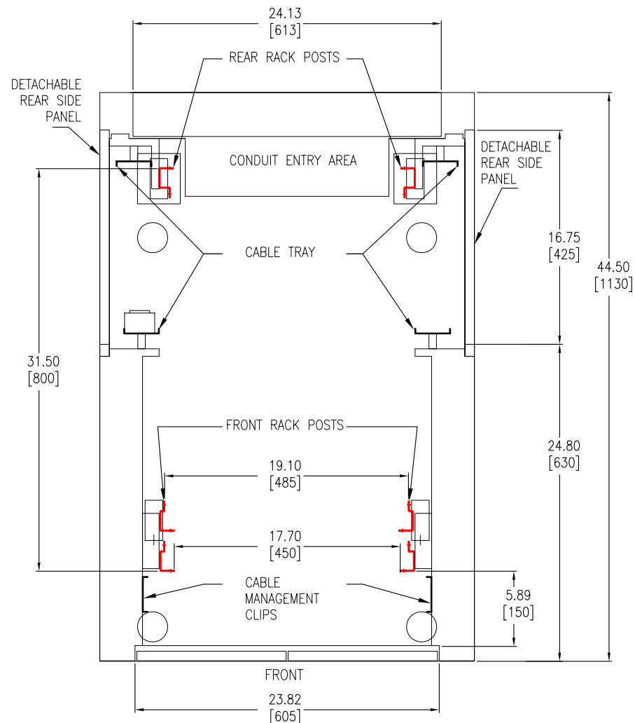
INTERNAL-BOTTOM VIEW (LOOKING FROM TOP)
