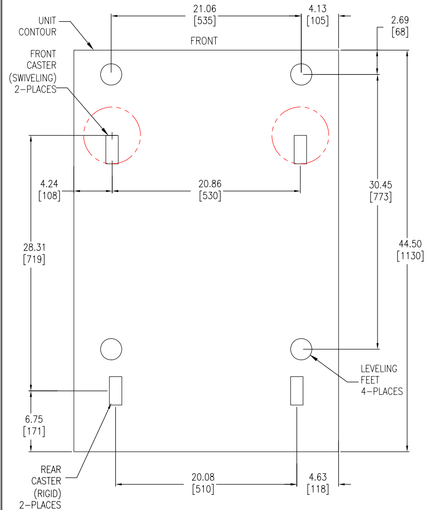
BOTTOM VIEW
