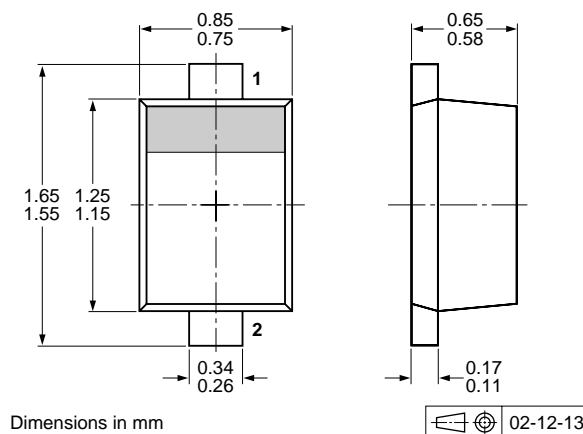
Fig 8. Package outline PESD3V3L1UB (SOD523/SC-79)
