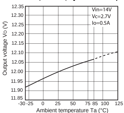
Fig.24 Output Voltage vs. Ambient Temperature (PQ120RDA1SZH)
