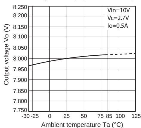
Fig.22 Output Voltage vs. Ambient Temperature (PQ080RDA1SZH)
