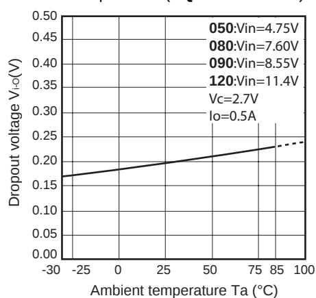
Fig.25 Dropout Voltage vs. Ambient Temperature (PQxxxRDA1SZH)
