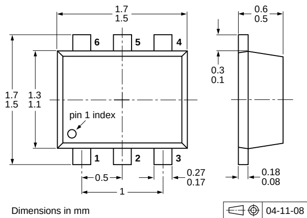
Fig 10. Package outline PEMB2 (SOT666)
