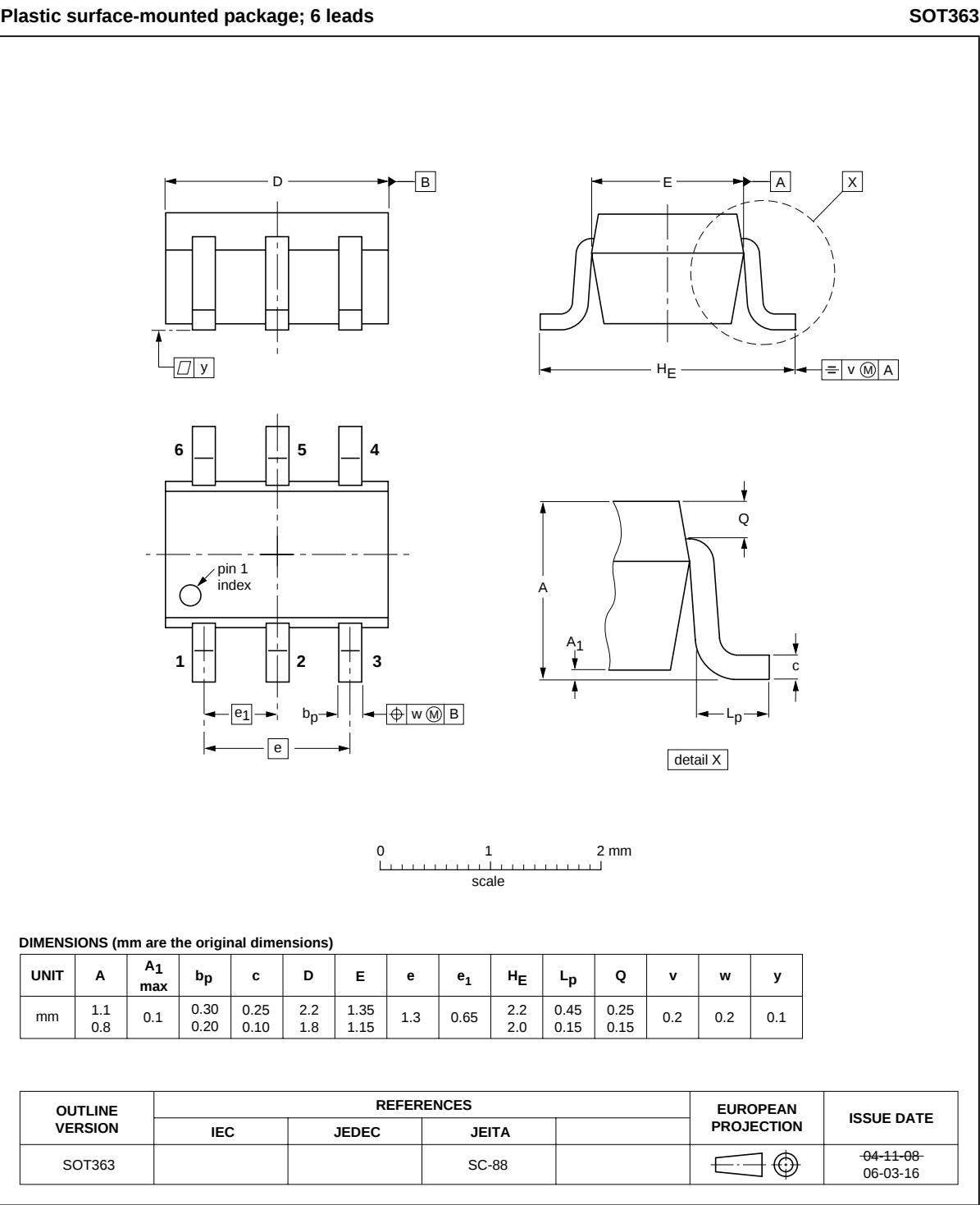
Fig 5. Package outline SOT363 (SC-88)
