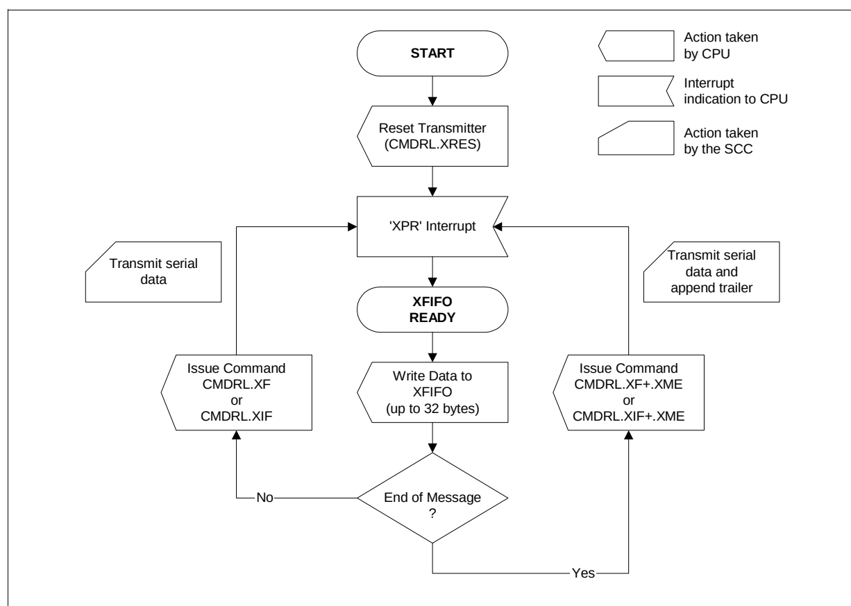
Figure 53 Interrupt Driven Data Transmission (Flow Diagram)
