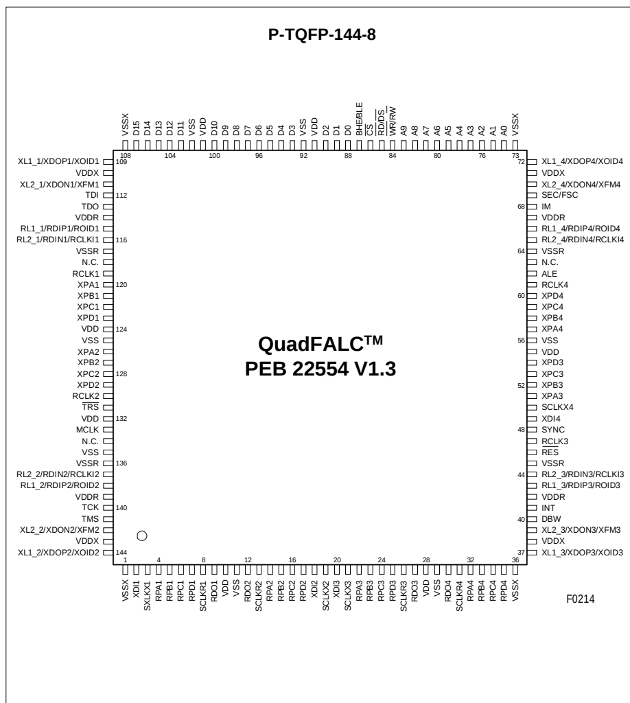
Figure 4 Pin Configuration
