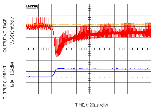
Figure 4. Transient Response to Dynamic Load Change from 50% to 100% at 12Vin, C_{out}= 3 \times 47\mu\text{F} + 6 \times 330\mu\text{F} , C_{Tune}=47\text{nF} , R_{Tune}=180\Omega
