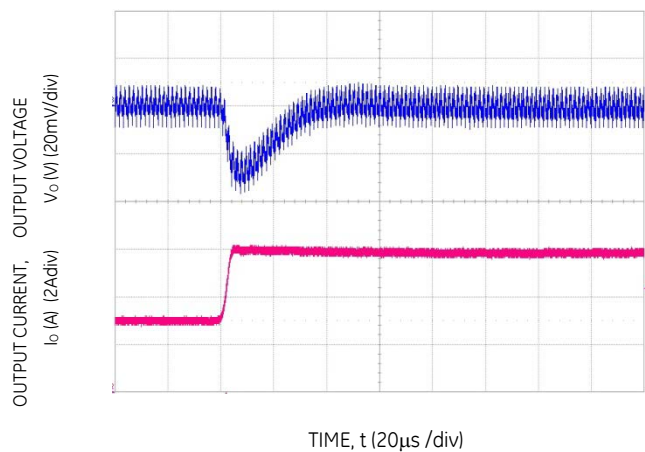
Figure 16. Transient Response to Dynamic Load Change from 50% to 100% at 12V in , C out = 1x47μF + 1x330μF, C Tune =4700pF, R Tune =178
