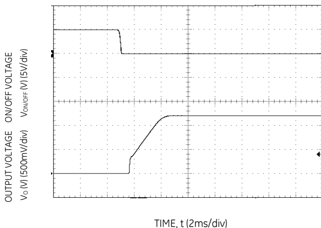
Figure 1. Typical Start-up Using On/Off Voltage ( I_o = I_{o,max} ).
