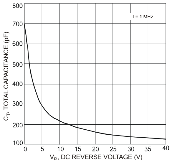
Fig. 5 Total Capacitance vs. Reverse Voltage, Per Element
