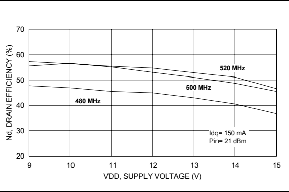
Figure 24. Drain efficiency vs. supply voltage
