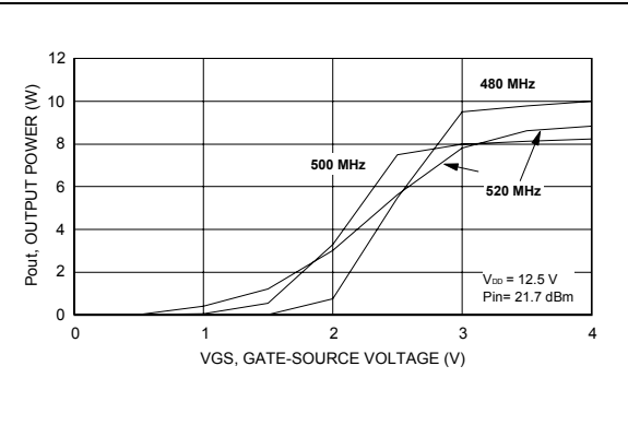
Figure 14. Output power vs. gate-source voltage
