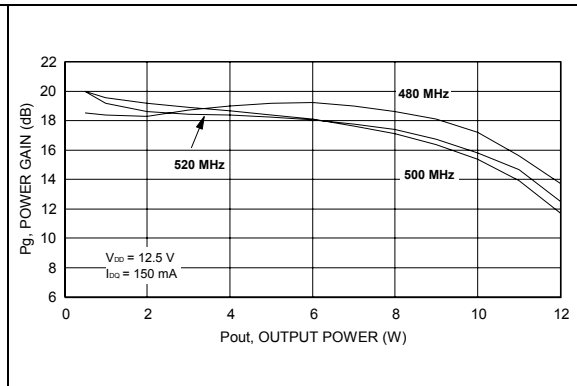
Figure 7. Power gain vs. output power
