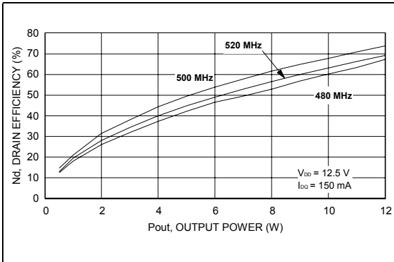
Figure 8. Drain efficiency vs. output power
