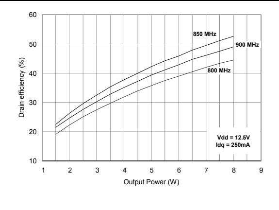
Figure 15. Drain efficiency vs. output power
