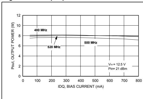
Figure 21. Output power vs. bias current
