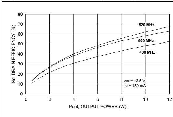
Figure 19. Drain efficiency vs. output power
