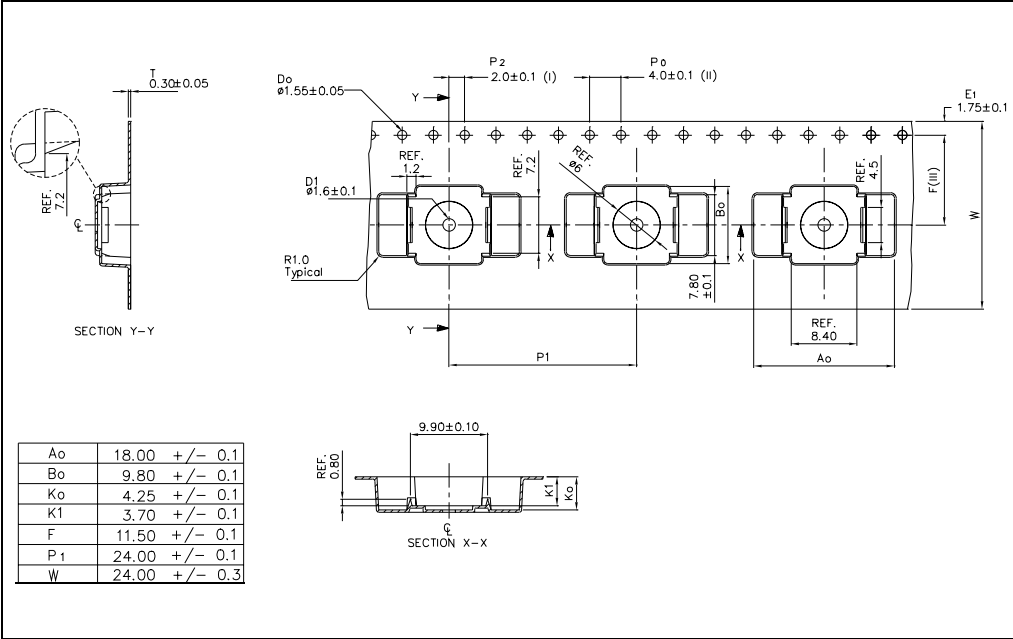
Figure 31. Reel information
