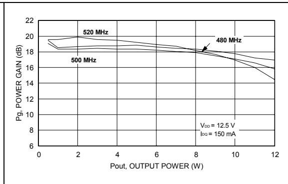
Figure 18. Power gain vs. output power
