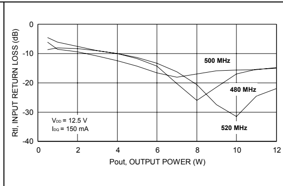
Figure 9. Input return loss vs. output power
