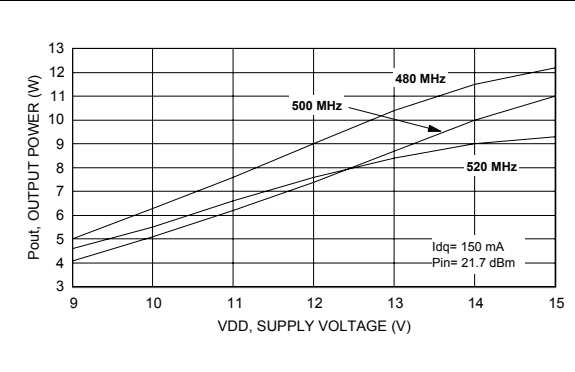
Figure 12. Output power vs. supply voltage
