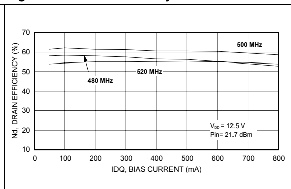
Figure 11. Drain efficiency vs. bias current
