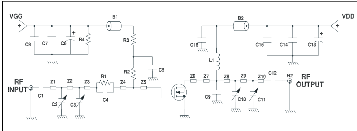
Figure 26. Test circuit schematic
