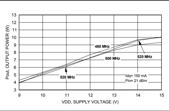
Figure 23. Output power vs. supply voltage
