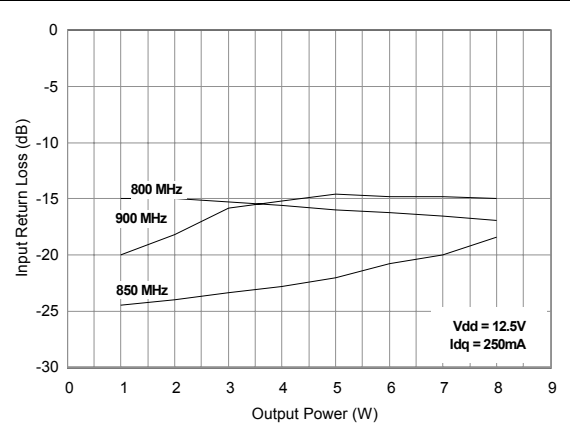
Figure 16. Input return loss vs. output power
