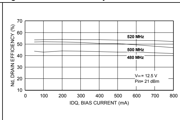
Figure 22. Drain efficiency vs. bias current
