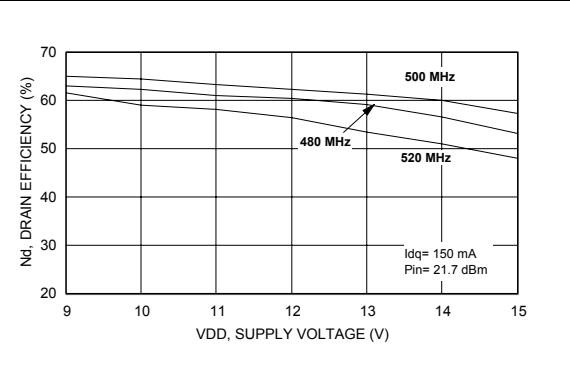
Figure 13. Drain efficiency vs. supply voltage
