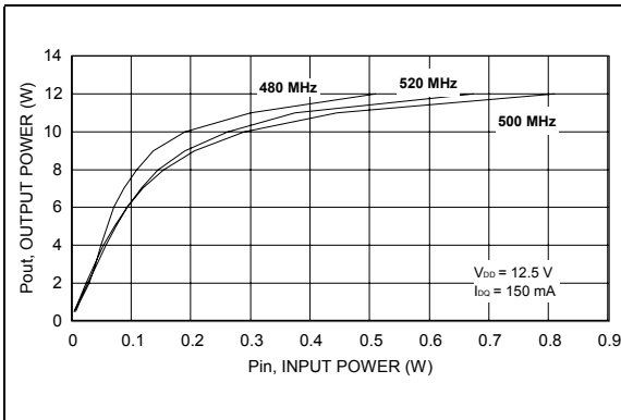
Figure 6. Output power vs. input power
