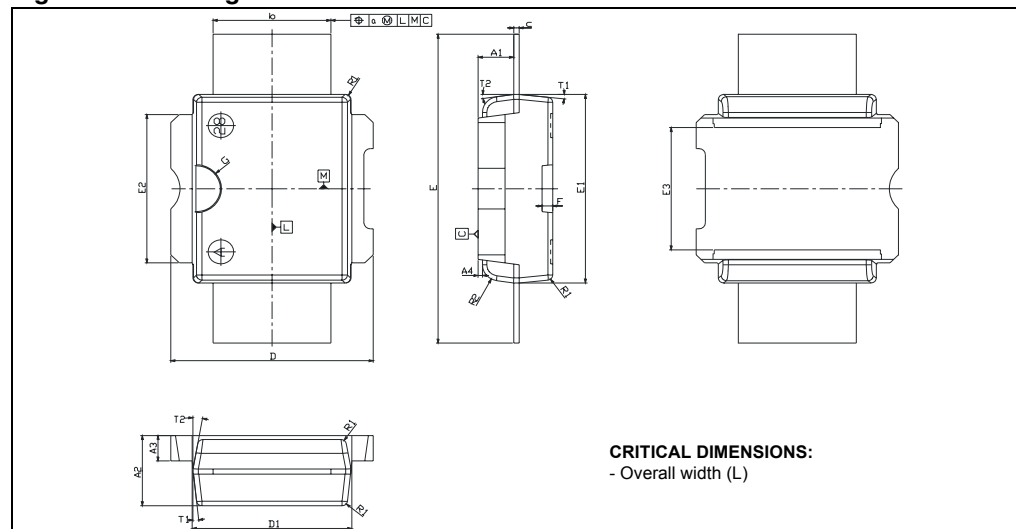
Figure 29. Package dimensions
