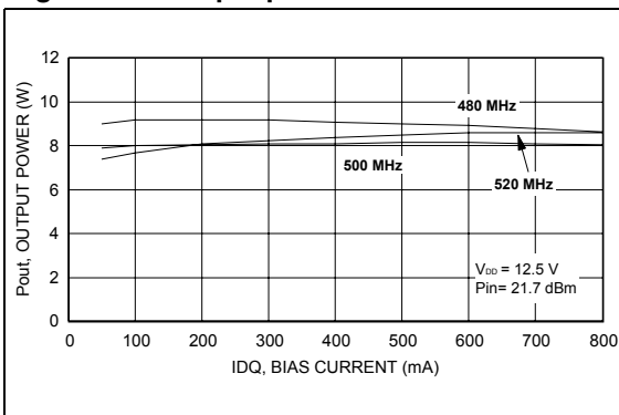
Figure 10. Output power vs. bias current
