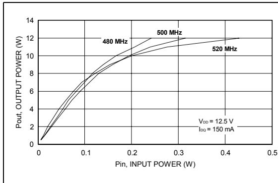
Figure 17. Output power vs. input power
