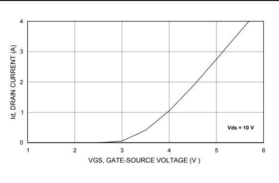
Figure 4. Drain current vs. gate-source voltage
