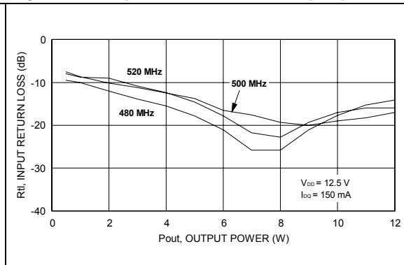
Figure 20. Input return loss vs. output power
