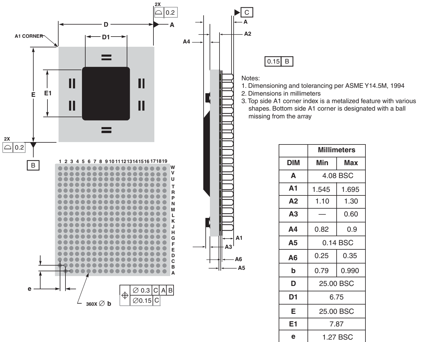
Figure 8-10. Mechanical Dimensions and Bottom Surface Nomenclature of PC755 (CI-CGA) (GS)
