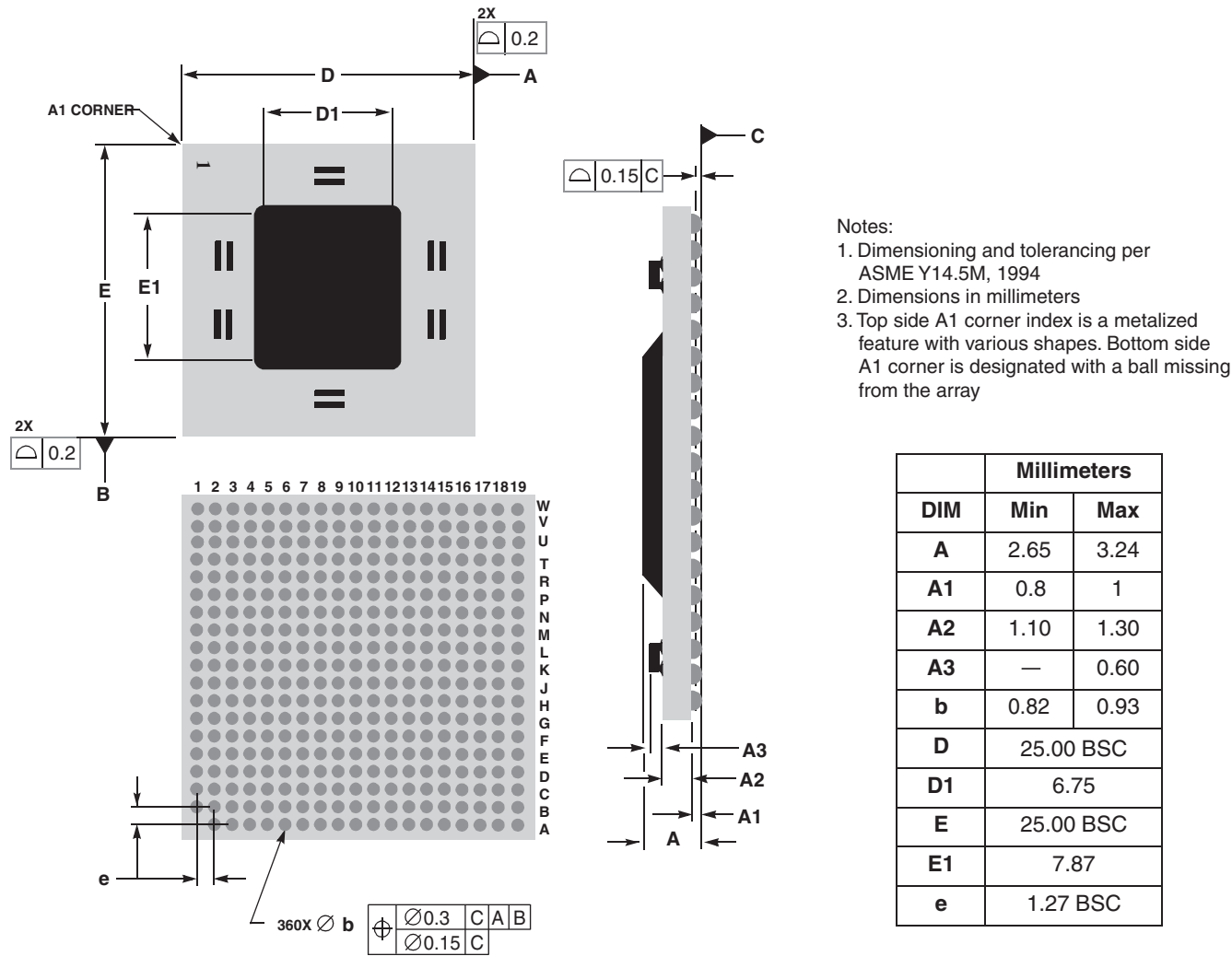
Figure 8-6. Mechanical Dimensions and Bottom Surface Nomenclature of PC755 (HiTCE) (GH)
