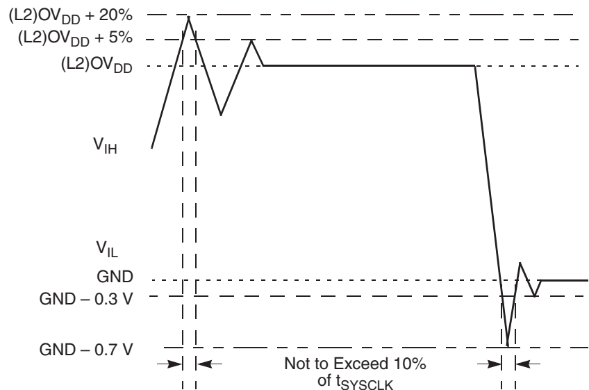
Figure 5-1. Overshoot/Undershoot Voltage
