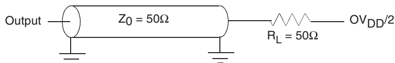
Figure 5-10. AC Test Load for the JTAG Interface
