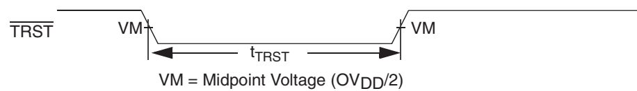
Figure 5-12. \overline{TRST} Timing Diagram
