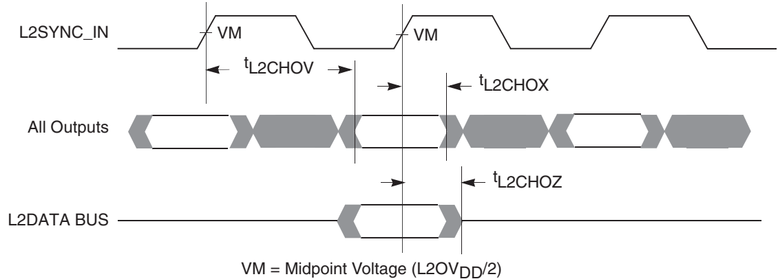
Figure 5-8. L2 Bus Output Timing Diagrams
