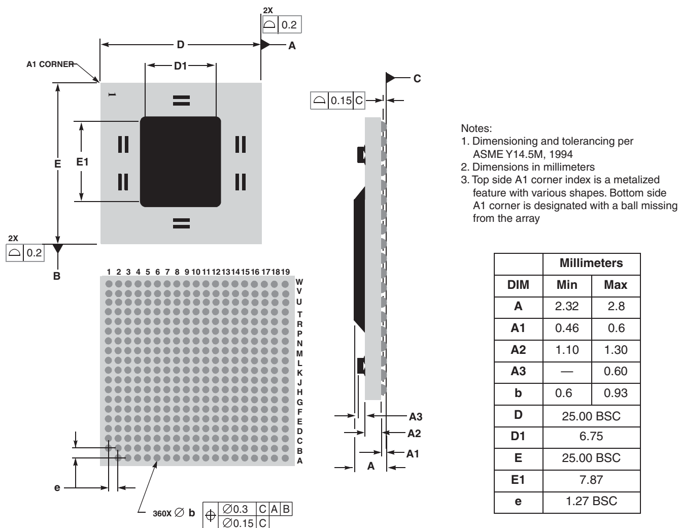
Figure 8-7. Mechanical Dimensions and Bottom Surface Nomenclature of PC755 (HiTCE-RoHS) (SH)
