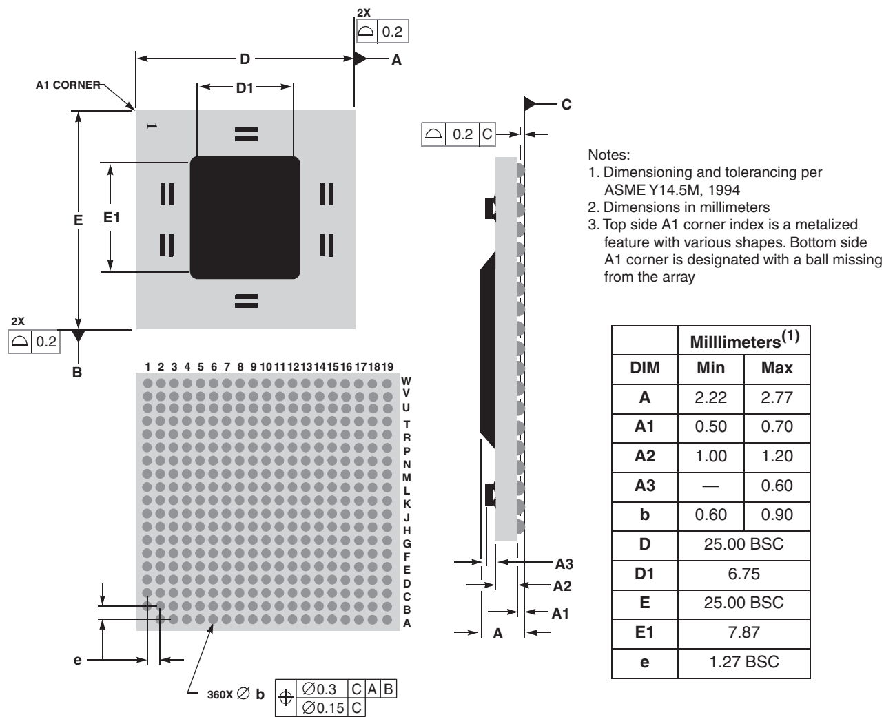
Figure 8-4. Mechanical Dimensions and Bottom Surface Nomenclature of the PC755 PBGA (ZF)
