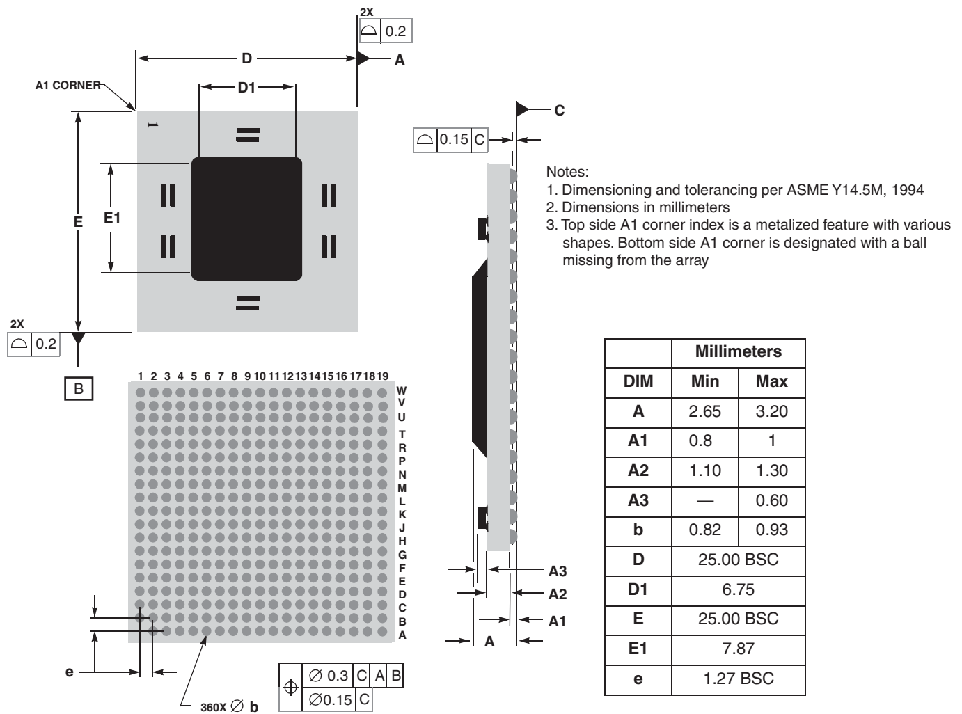
Figure 8-5. Mechanical Dimensions and Bottom Surface Nomenclature of PC755 (CBGA) (G)
