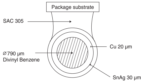
Figure 8-9. Polymer Solder Spheres Composition
