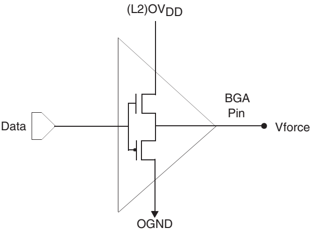
Figure 9-3. Alternate Driver Impedance Measurement Circuit
