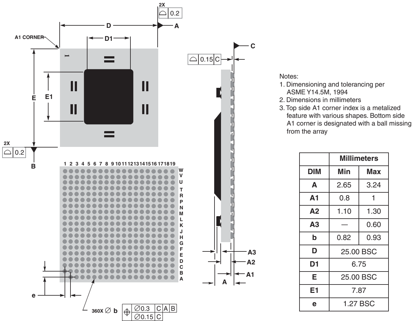
Figure 8-8. Mechanical Dimensions and Bottom Surface Nomenclature of PC755 (HiTCE-RoHS) (PH)
