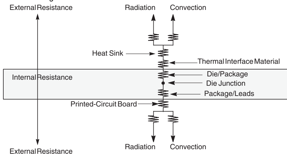
Figure 9-6. C4 Package with Heat Sink Mounted to a Printed-Circuit Board
