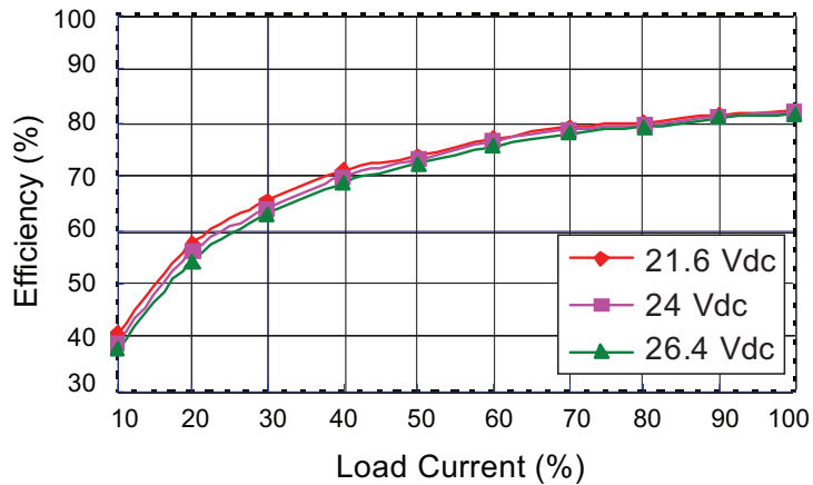
PCN1-S24-S15-M Efficiency Curve (Efficiency vs. Line Voltage and Load Current)
