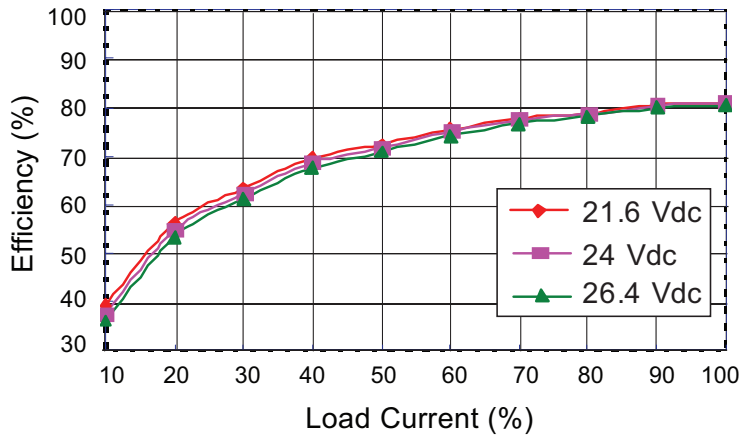
PCN1-S24-D12-M Efficiency Curve (Efficiency vs. Line Voltage and Load Current)
