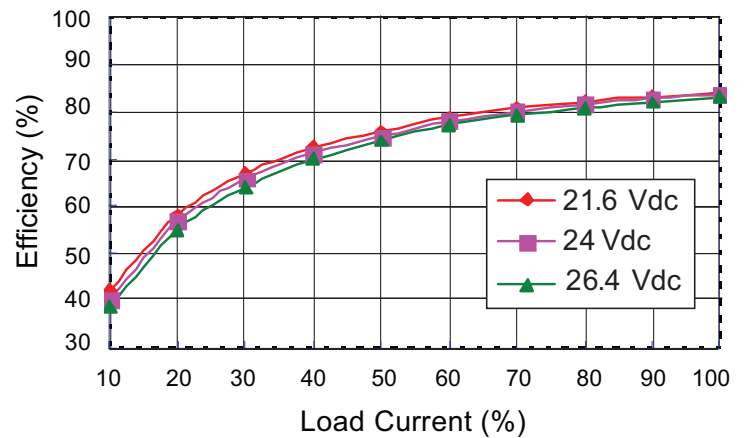
PCN1-S24-S12-M Efficiency Curve (Efficiency vs. Line Voltage and Load Current)
