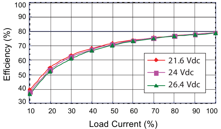
PCN1-S24-D5-M Efficiency Curve (Efficiency vs. Line Voltage and Load Current)
