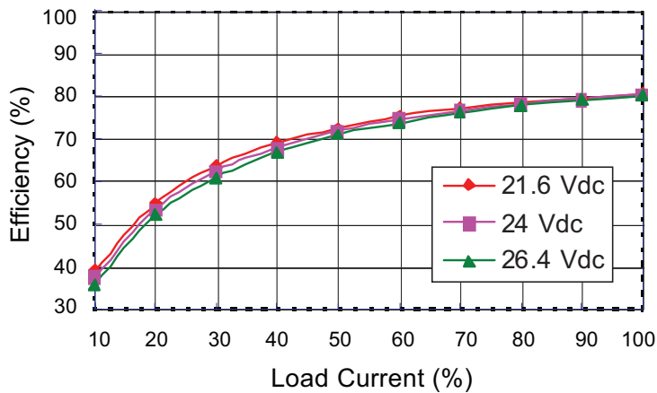
PCN1-S24-S5-M Efficiency Curve (Efficiency vs. Line Voltage and Load Current)
