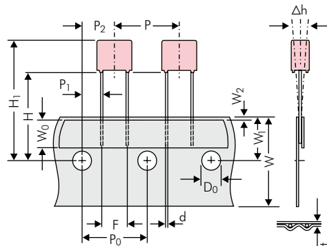
Diagram 1: PCM 2.5/5/7.5mm
