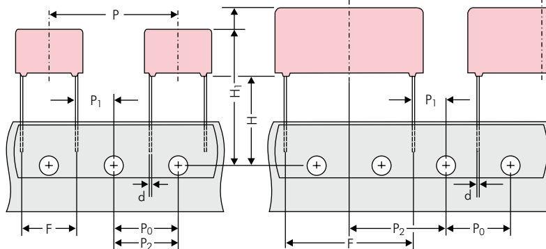
Diagram 2: PCM 10/15 mm
