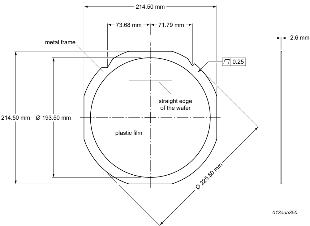
Fig 37. Film Frame Carrier (FFC) for 6 inch wafer (PCF2123U/10AA/1)
