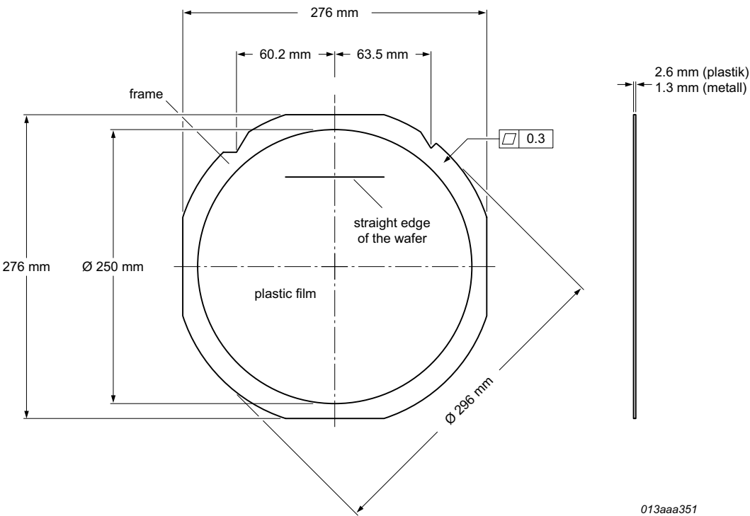
Fig 38. Film Frame Carrier (FFC) for 8 inch wafer (PCF2123U/12AA/1 and PCF2123U/12HA/1)
