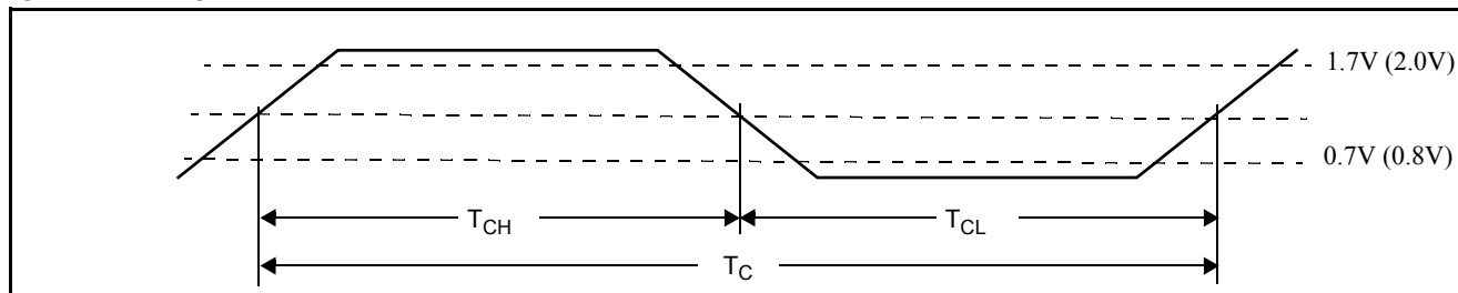
Figure 5. Timing Waveform
