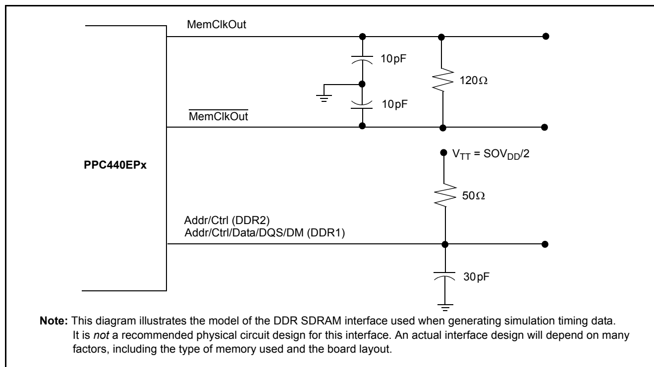
Figure 9. DDR SDRAM Simulation Signal Termination Model
