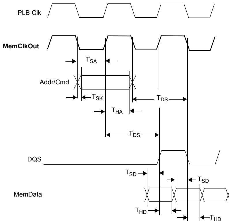
Figure 10. DDR SDRAM Write Cycle Timing
