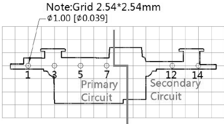
Top View PCB Layout
