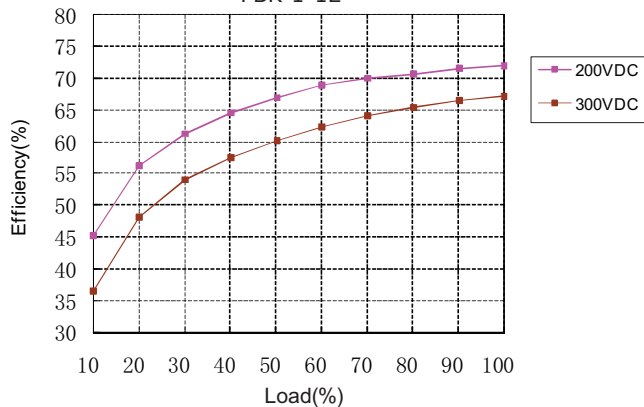
efficiency vs. load PBK-1-12
