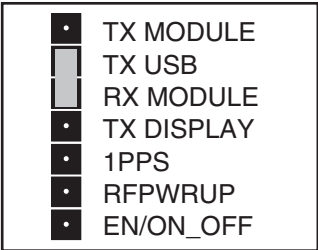
Figure 5: Jumper Configuration
