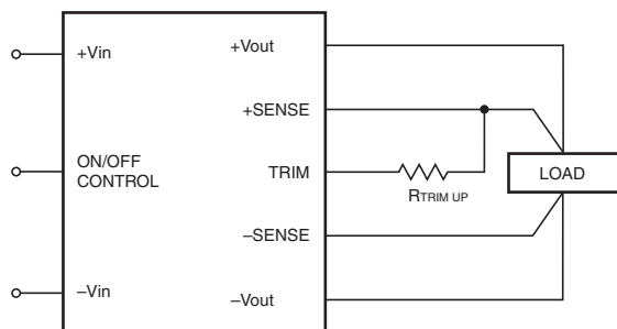
Figure 4. Trim Connections To Increase Output Voltages Using Fixed Resistors
