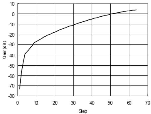
9. Gain Step
