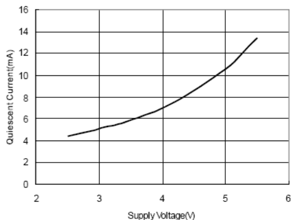
16. Quiescent Current
