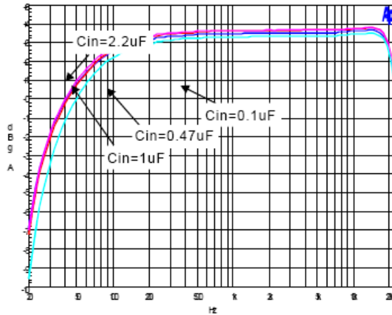
7. Frequency Response
