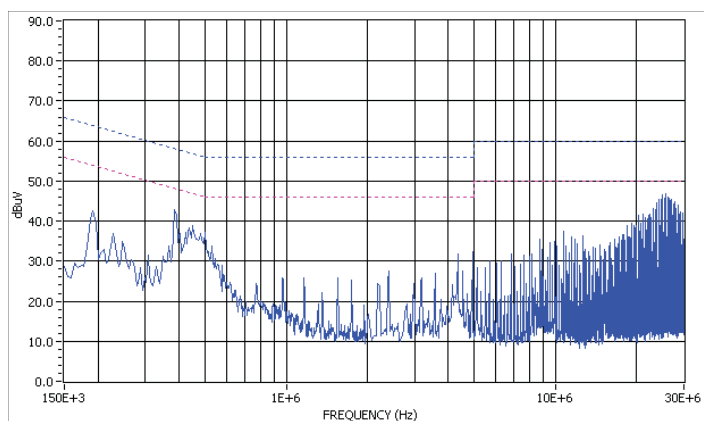
Graph 1. Conducted emissions performance, Positive Line, CISPR 22, Class A, full load
