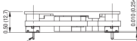
Bottom Pin Side View
