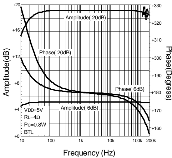
Frequency Response
