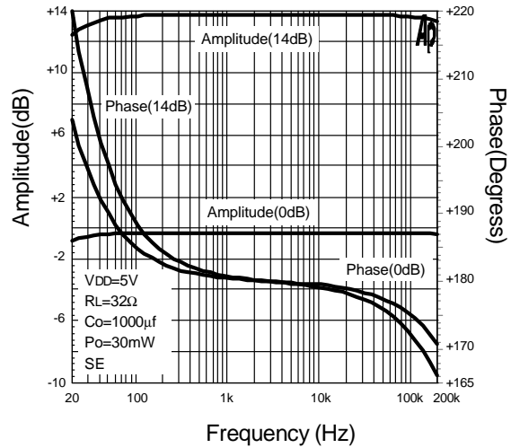
Frequency Response
