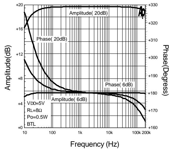
Frequency Response
