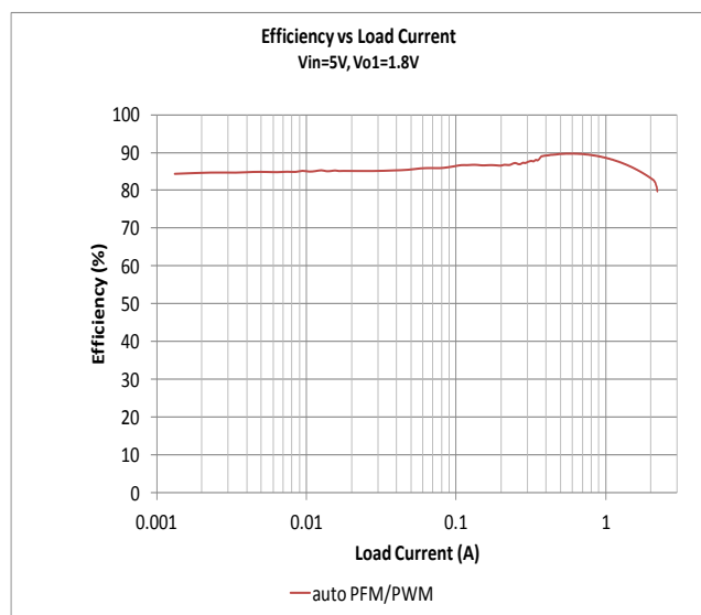
Figure 7. Channel 1 Efficiency
