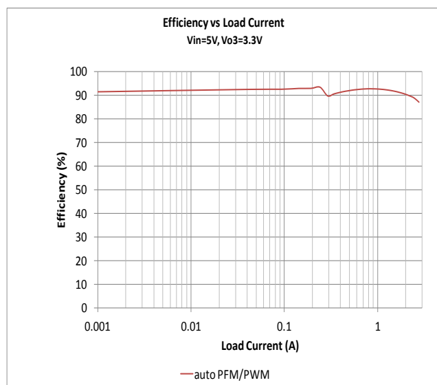
Figure 9. Channel 3 Efficiency
