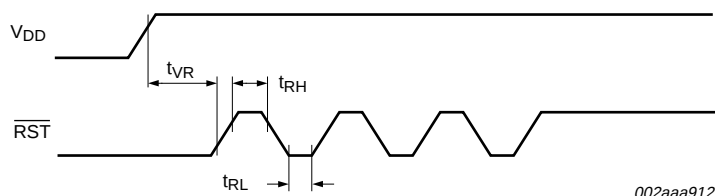
Fig 24. ISP entry waveform
