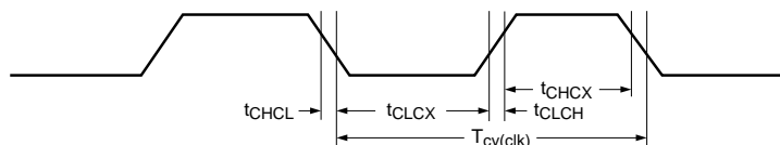
Fig 32. External clock drive waveform
