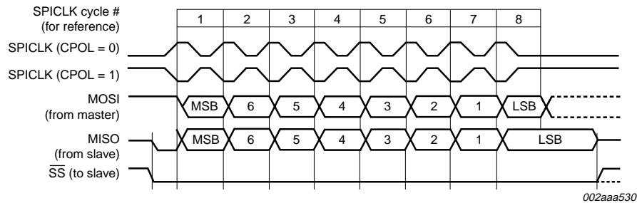
Fig 18. SPI transfer format with CPHA = 1
