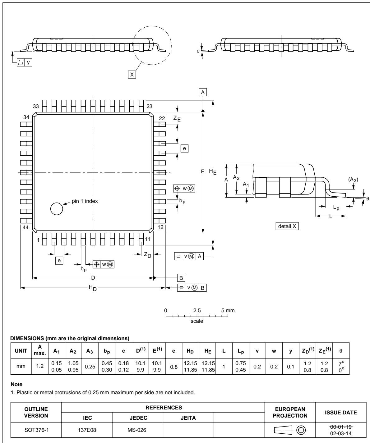
Fig 39. Package outline SOT376-1 (TQFP44)
