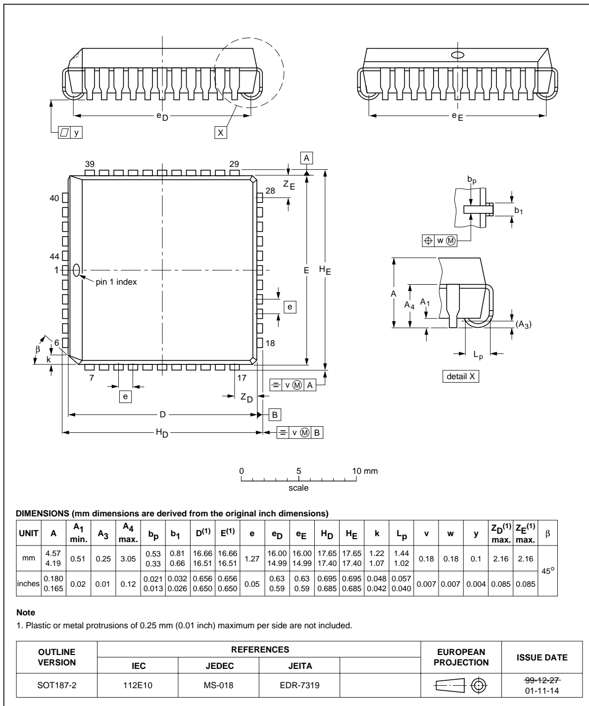
Fig 38. Package outline SOT187-2 (PLCC44)
