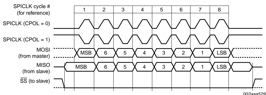
Fig 17. SPI transfer format with CPHA = 0
