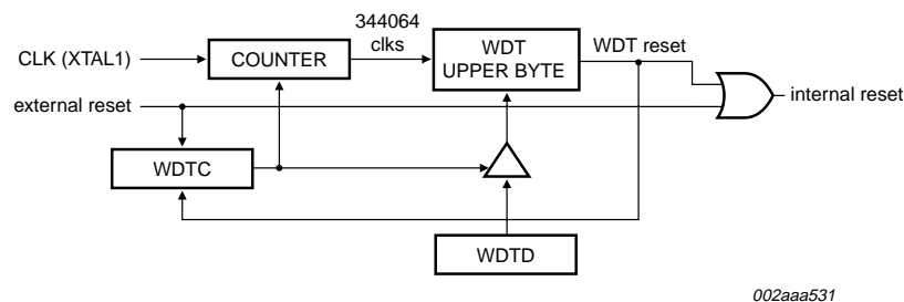
Fig 19. Block diagram of programmable WDT
