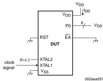
Fig 40. I_{DD} test condition, Idle mode
