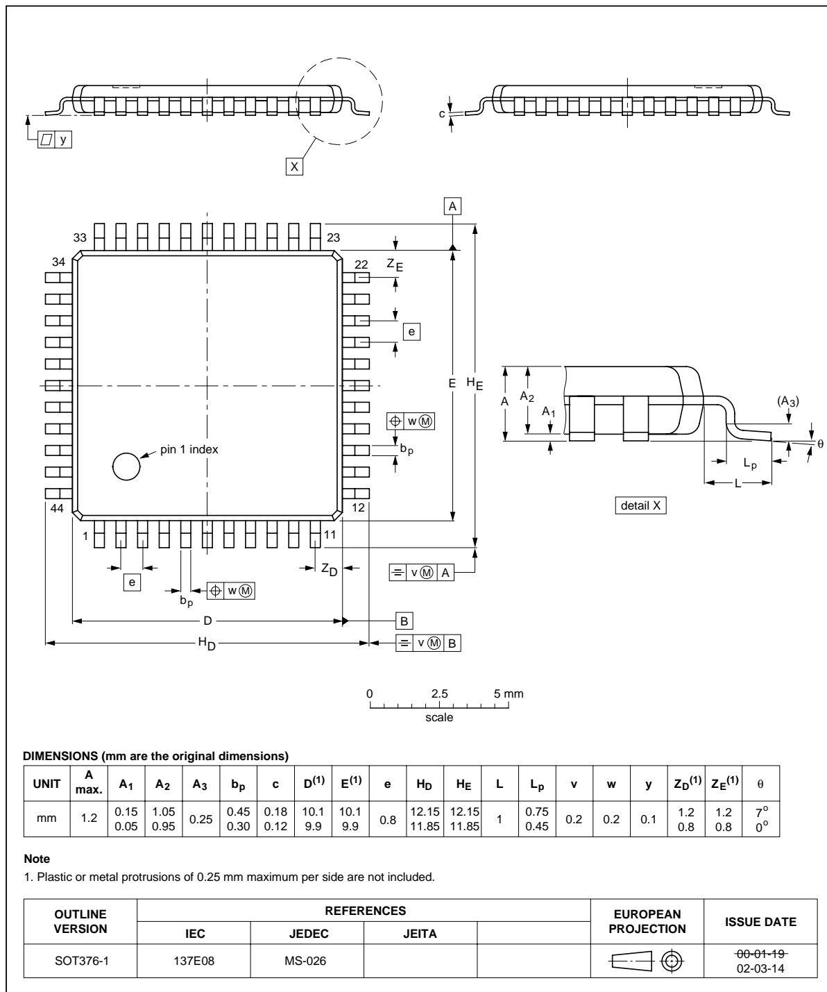
Fig 42. Package outline SOT376-1 (TQFP44)
