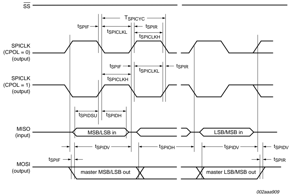
Fig 35. SPI master timing (CPHA = 1)
