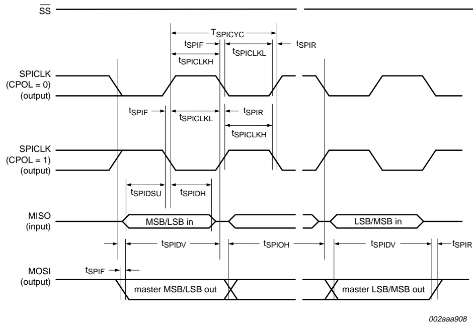
Fig 34. SPI master timing (CPHA = 0)
