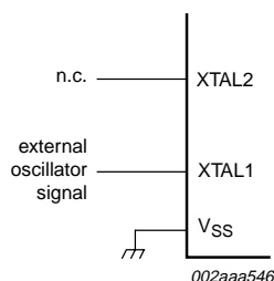
Fig 27. Oscillator characteristics (external clock drive)
