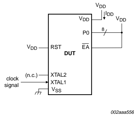
Fig 39. I_{DD} test condition, Active mode
