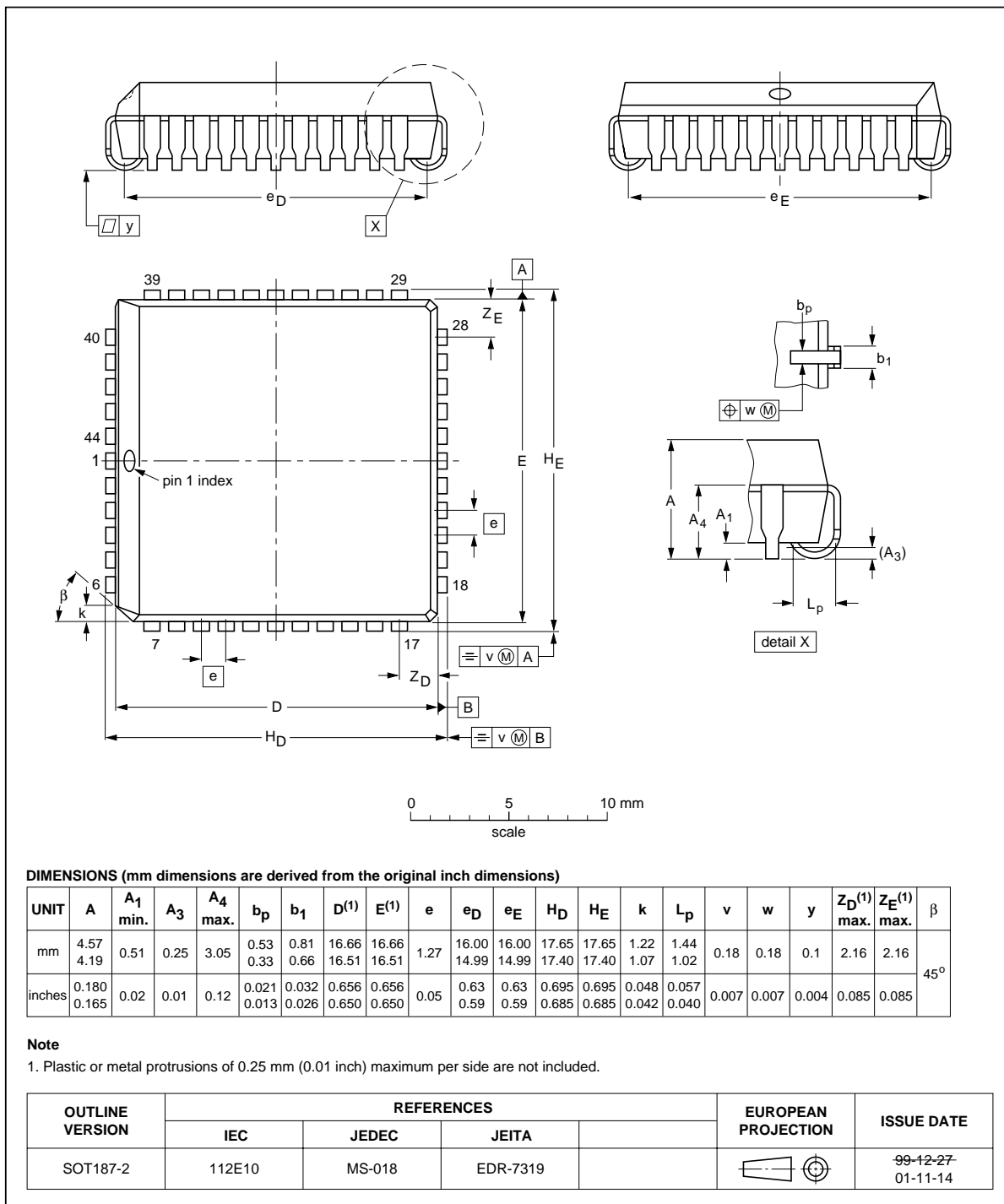
Fig 43. Package outline SOT187-2 (PLCC44)
