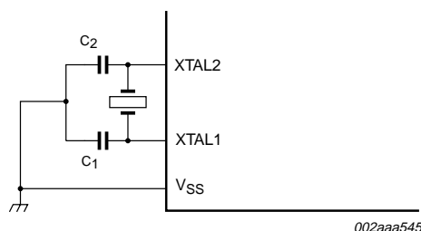
Fig 26. Oscillator characteristics (using the on-chip oscillator)
