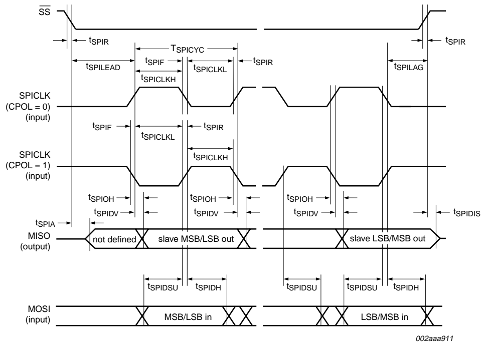
Fig 37. SPI slave timing (CPHA = 1)
