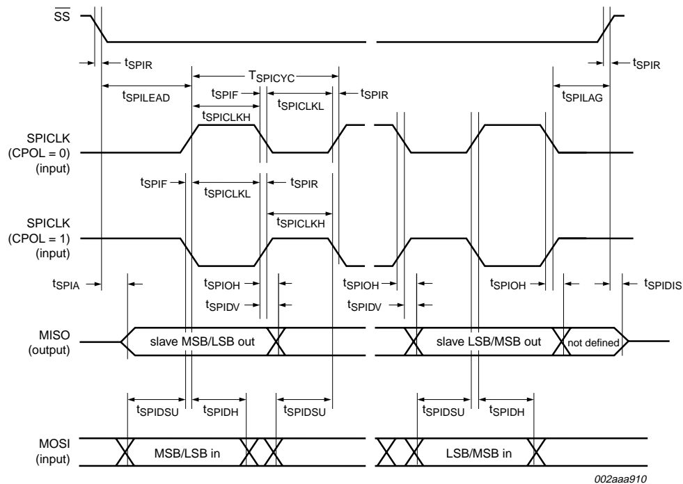
Fig 36. SPI slave timing (CPHA = 0)
