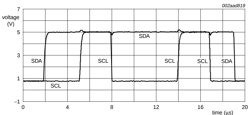
Fig 11. Clock and data signal output to a slave from Sx/Sy of a P82B96 replacing one of the P82B715s
