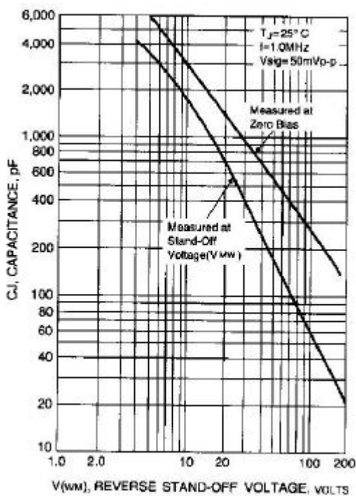
Fig. 4-TYPICAL JUNCTION
