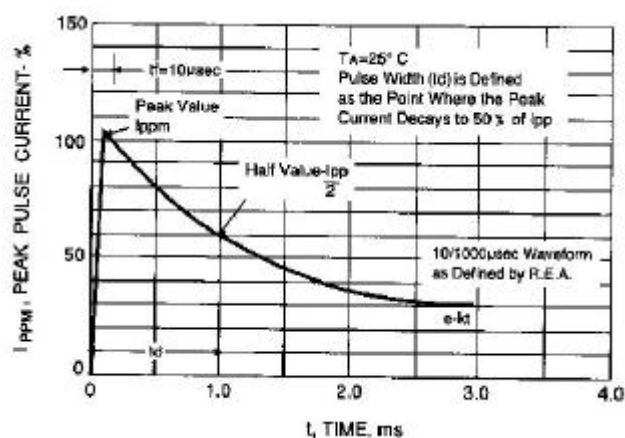
Fig. 3-PULSE WAVEFORM CAPACITANCE
