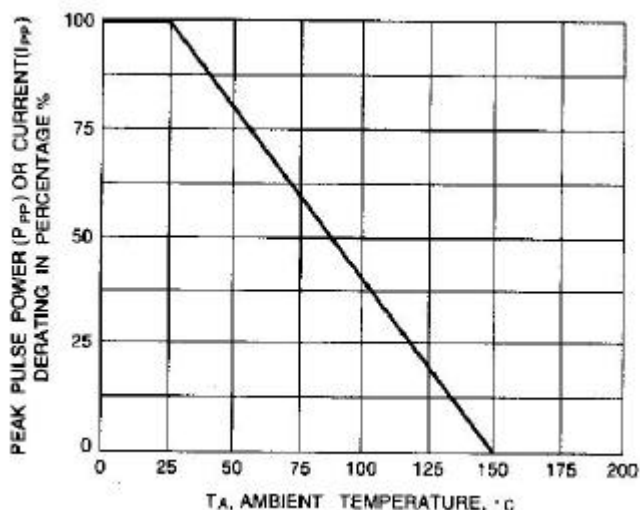
Fig. 2-PULSE RATING CURVE
