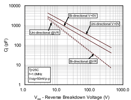
Figure 4 - Typical Junction Capacitance Uni-Directional
