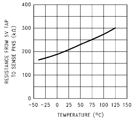
Divider Resistance
