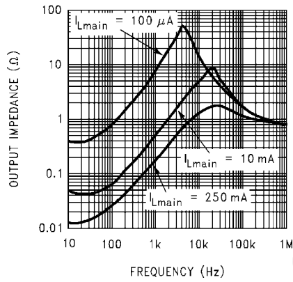
Output Impedance (Main Regulator)
