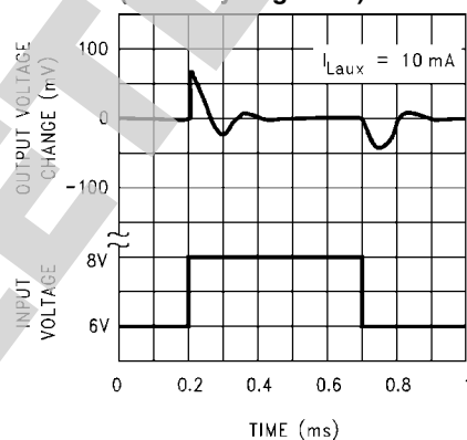
Line Transient Response (Auxiliary Regulator)
