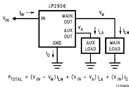
FIGURE 1. Current/Voltage Diagram
