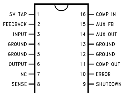
16-Pin DIP
