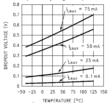
Dropout vs Temperature (Auxiliary Regulator)
