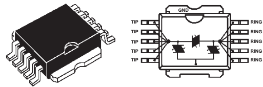
PowerSO-10 TM TLPxxM
