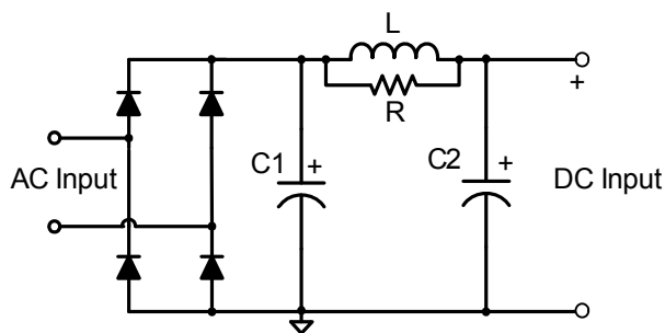
Figure 9: Input Filter
