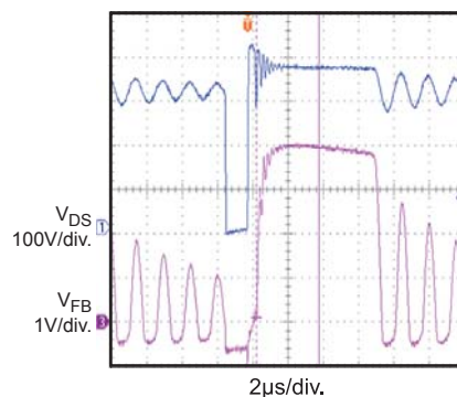
Normal Operation
