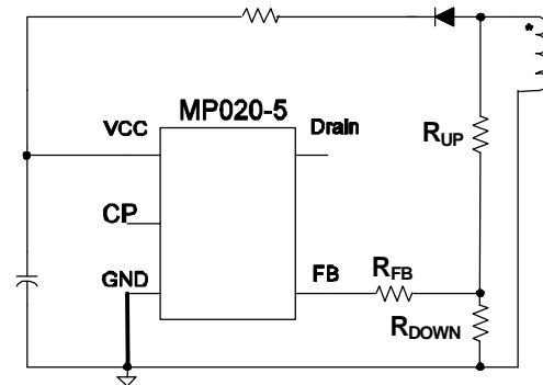
Figure 12: Feedback Resistor Divider Circuit
