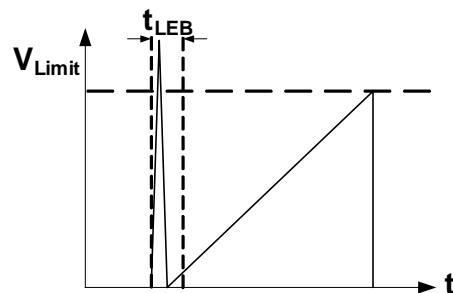
Figure 7: Leading-Edge Blanking
