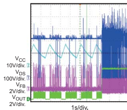
OVP Recovery
