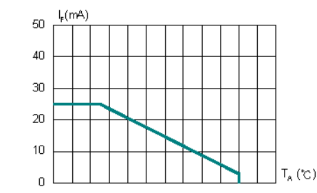
Fig.4 Allowable Forward Current vs. Ambient Temperature
