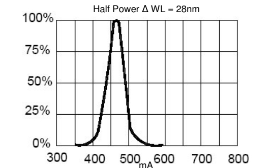
Relative Luminous Intensity vs. Wavelength
