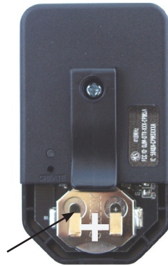
Figure 6: Battery Access
