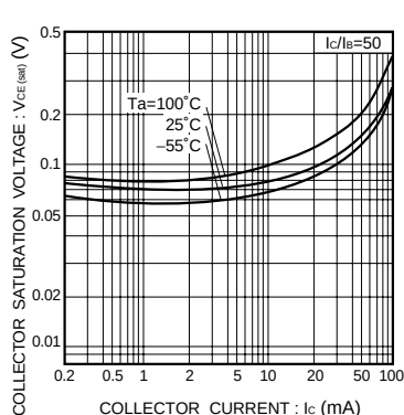
Fig.9 Collector-emitter saturation voltage vs. collector current ( III )
