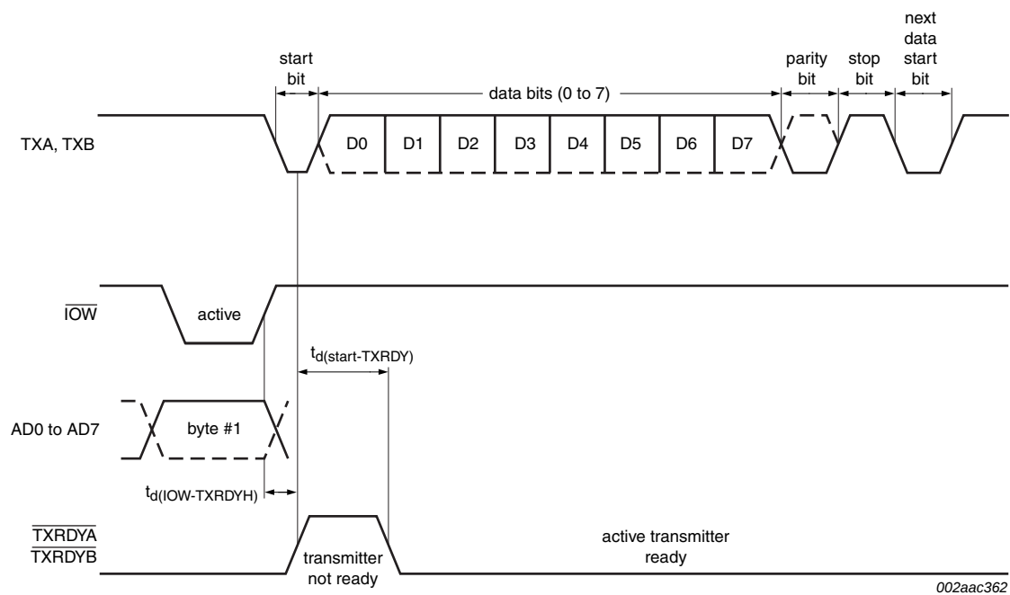
Fig 18. Transmit ready timing in non-FIFO mode
