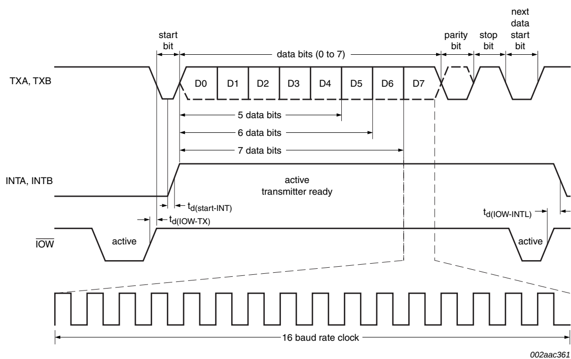
Fig 17. Transmit timing
