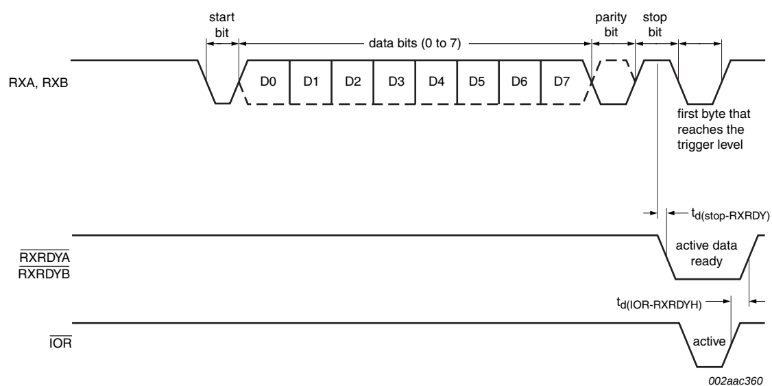
Fig 16. Receive ready timing in FIFO mode
