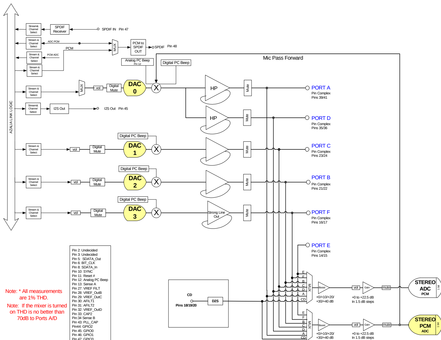
Figure 2. Functional Block Diagram STAC9221
