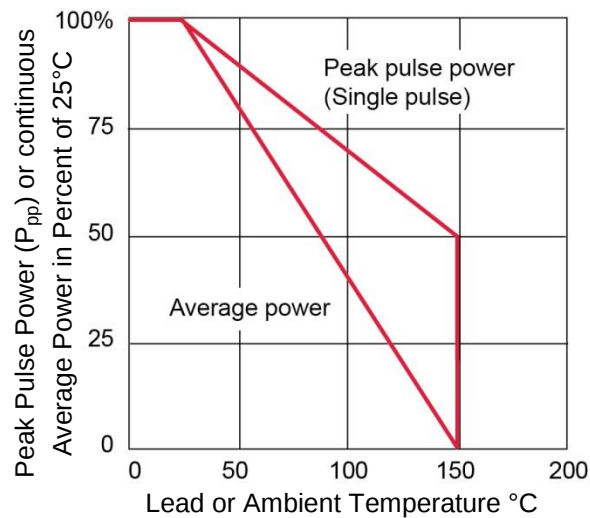
FIGURE 4 Derating Curve
