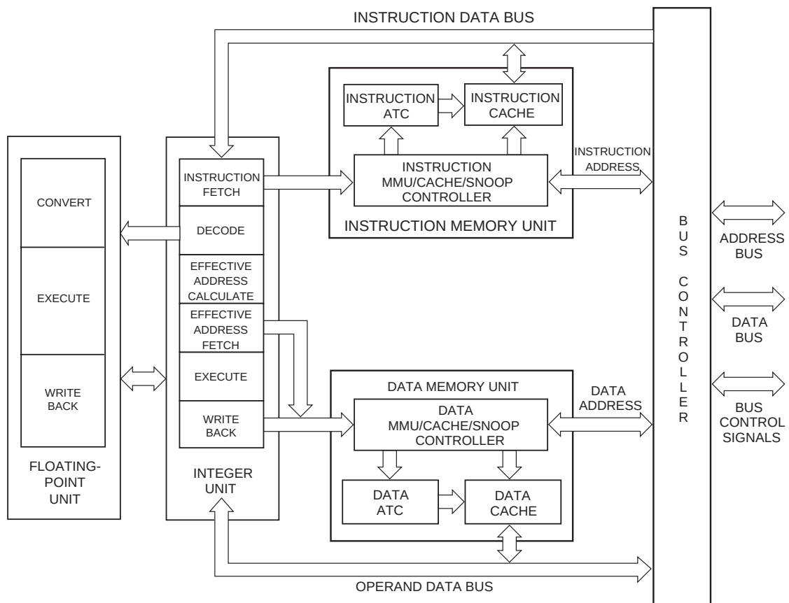
Figure 1. Block Diagram
