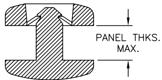
TYPICAL ASSEMBLY
