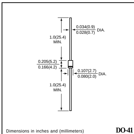
DO-41
