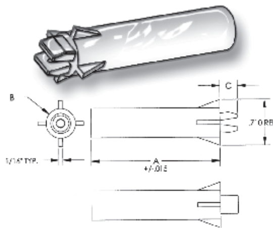
PART NUMBER 401034
