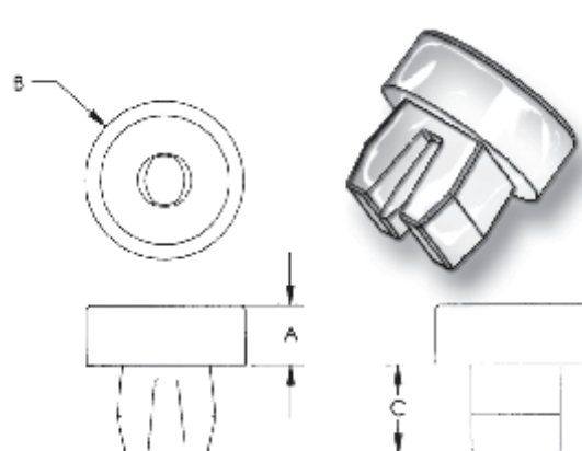
PART NUMBER 401021
