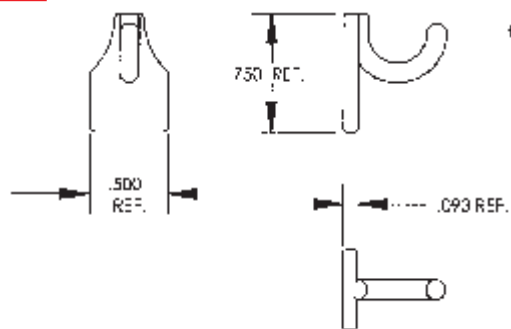
ITEM NUMBER DESCRIPTION 45INSTHOOK Ceiling Hanger Hook
