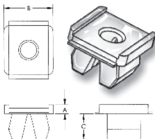
PART NUMBER 401025
