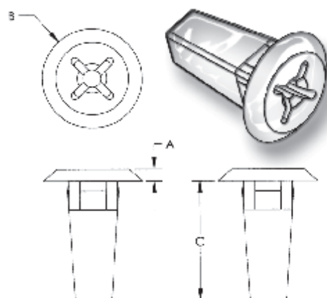
PART NUMBER 401018
