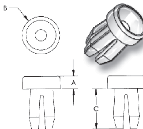
PART NUMBER 401012
