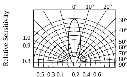
FIG.6 SENSITIVITY DIAGRAM
