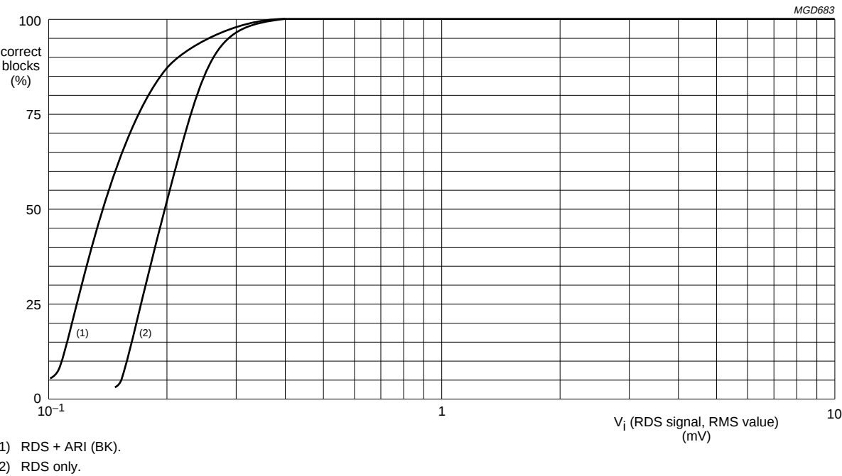
Fig.5 Typical RDS sensitivity.
