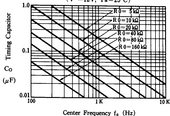
VCO Frequency
