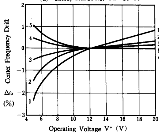
Center Frequency
