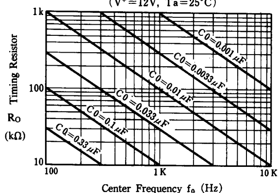
VCO Frequency
