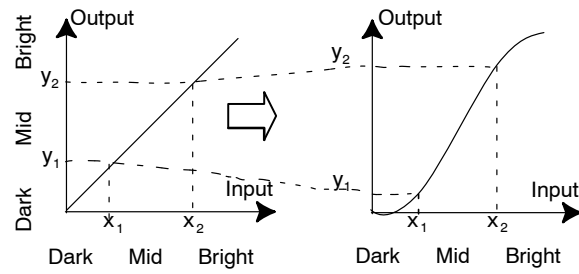
Figure 32. Tonal Mapping
