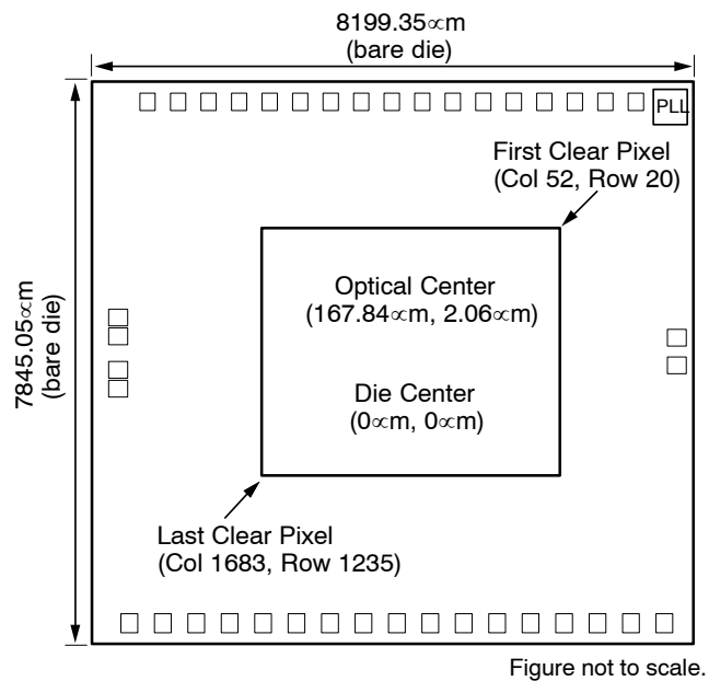
Figure 38. Optical Center Offset
